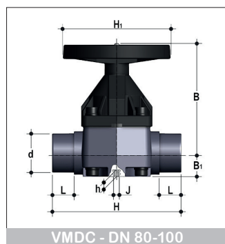
VMDC - DN 80-100
