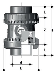
SSEIC DN 10-50
