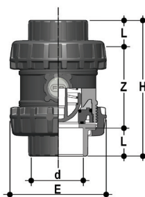
SSEIC DN 65-100
