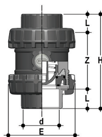
SSEIC DN 65-100
