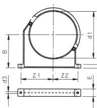
TYPE F
