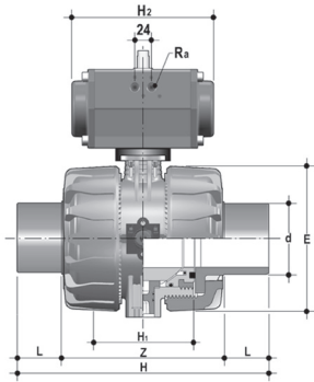
Dual Block VKD/CP
