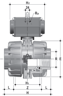
Dual Block VKDFV/CP
